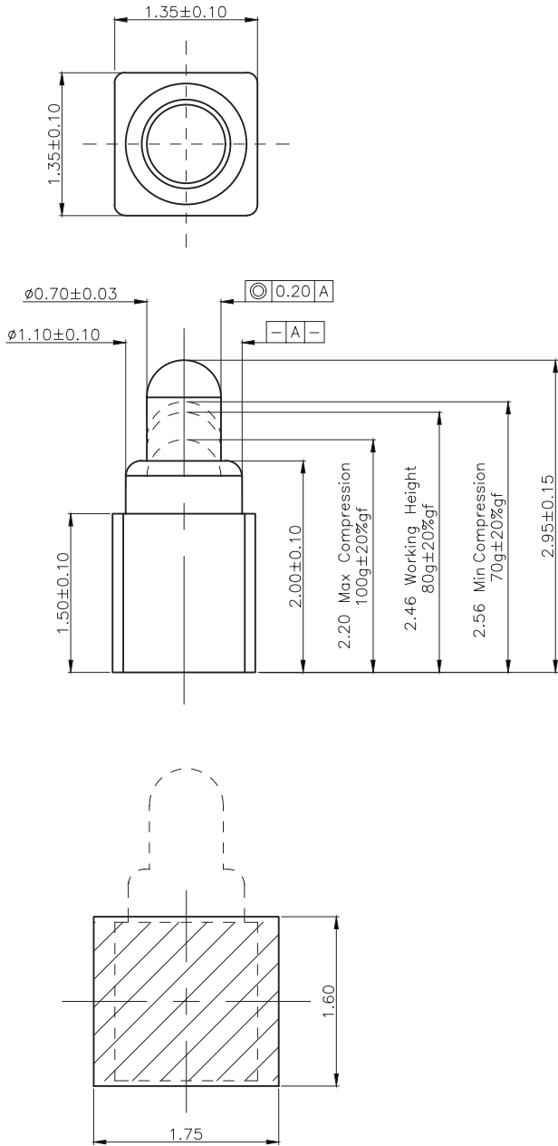
Recommended PCB Layout Top View
