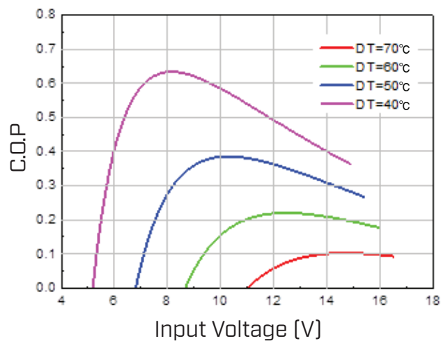
COP Vs. Input Voltage, V ( \Delta T=40\sim70^\circ\text{C} )
