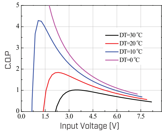
COP Vs. Input Voltage, V ( \Delta T=0\sim30^\circ\text{C} )
