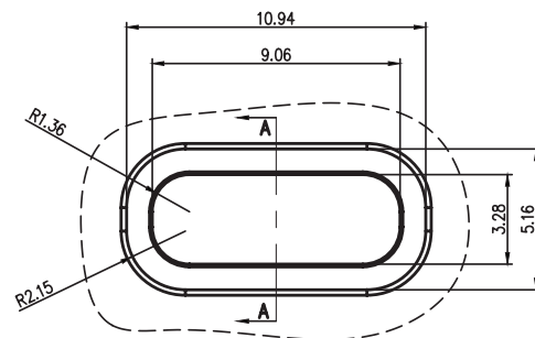
Recommended dimensions for enclosure cutouts
