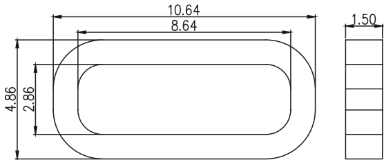
O-ring (P/N: OR-140)
