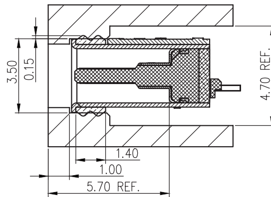
Recommended interference between the rubber ring and the housing
