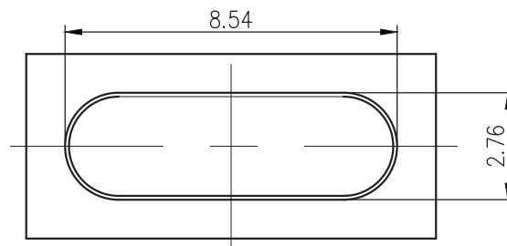
Chassis cutout dimensions
