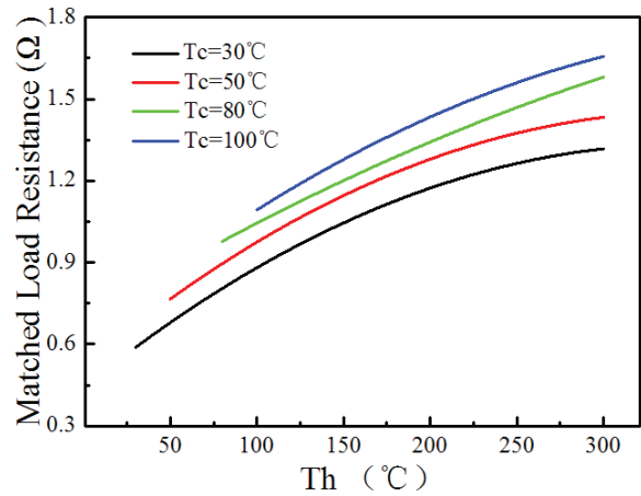
Matched Load Resistance Vs. Th
