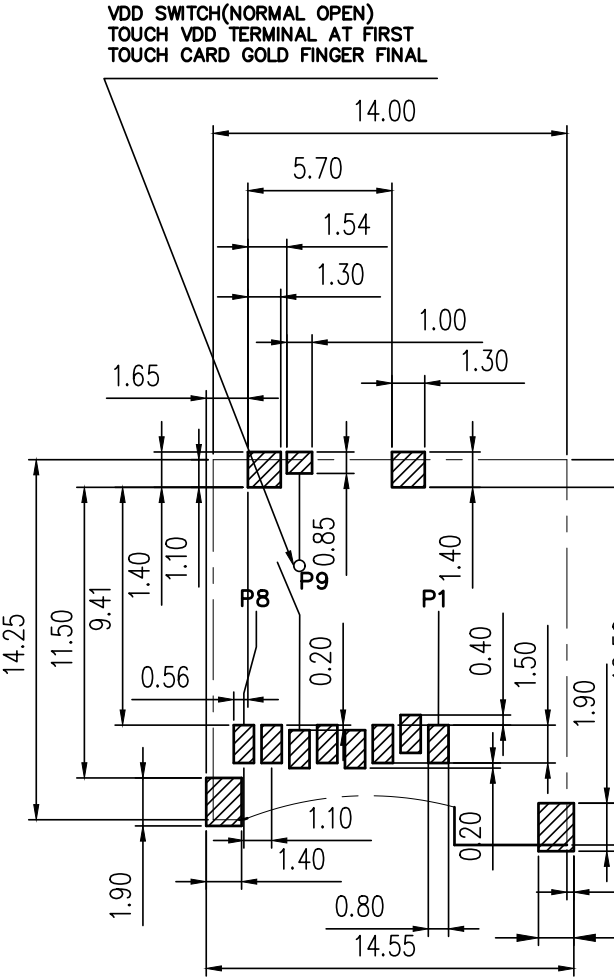
Recommended PCB Layout Top View
