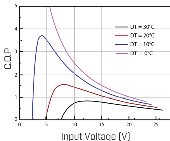
COP Vs. Input Voltage, V ( \Delta T = 0\text{--}30^\circ\text{C} )
