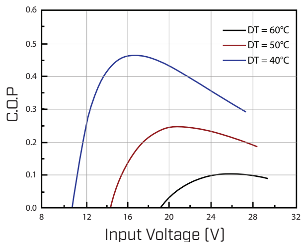
COP Vs. Input Voltage, V ( \Delta T = 40\text{--}60^\circ\text{C} )
