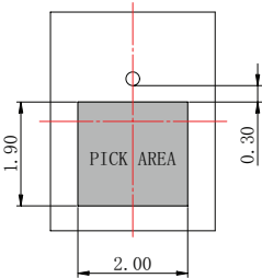
Recommended Vacuum Nozzle Pickup Top View
