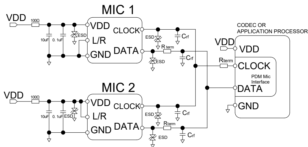
Double MIC
