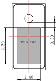
Recommended Vacuum Nozzle Pickup Top View
