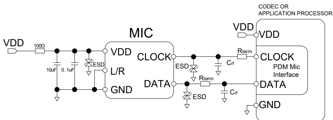
Single MIC
