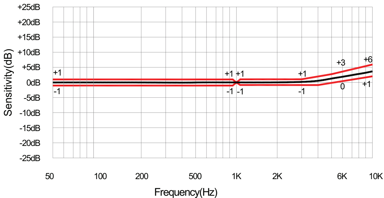
Frequency Response (0dB=1V/Pa)
