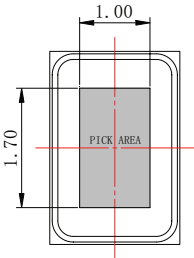
Recommended Vacuum Nozzle Pickup Top View
