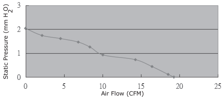
CFM-7015B-130-295
