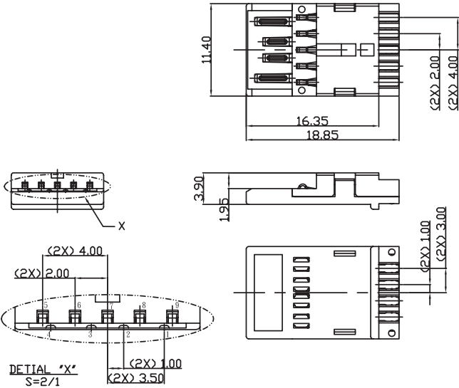
Connector
