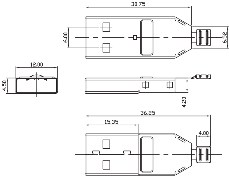
Bottom Cover
