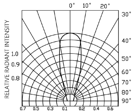
RADIATION DIAGRAM
