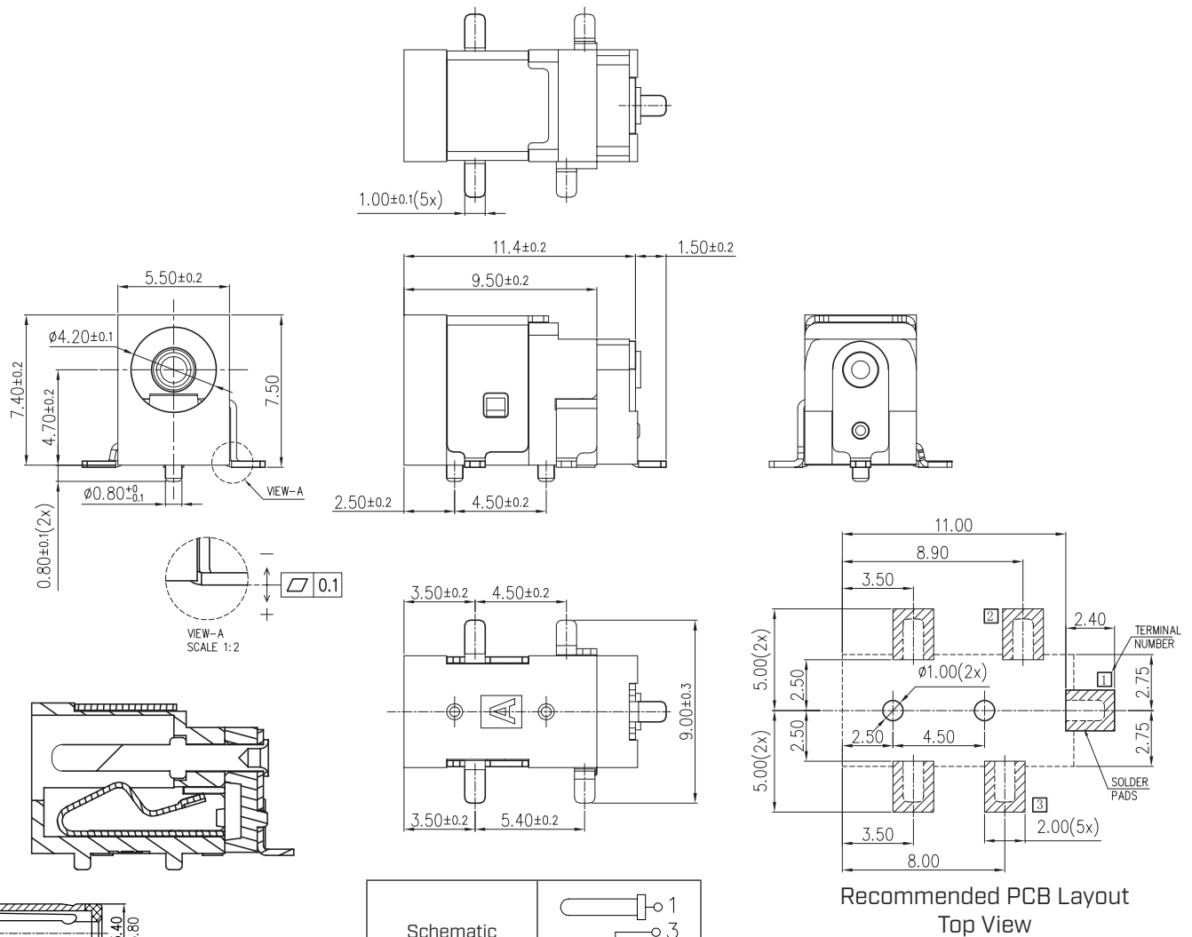
MATING PLUG Jack Insertion Depth: 6.6 mm
