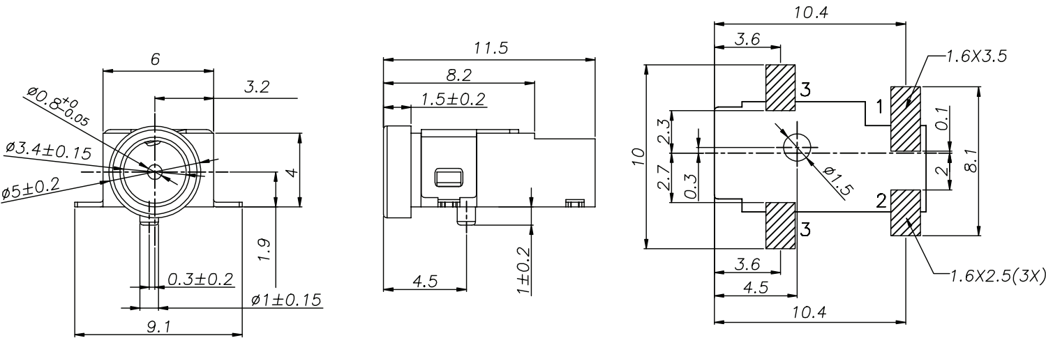
Recommended PCB Layout Top View
