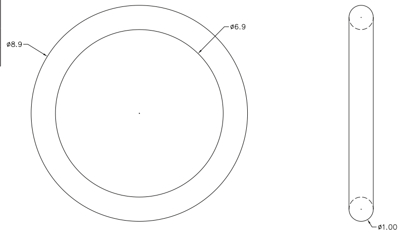
O-ring (P/N: OR-70)
