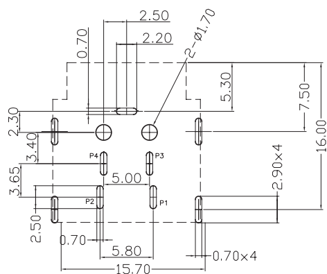
Recommended PCB Layout Top View (Date Codes prior to 03/03/2022)
