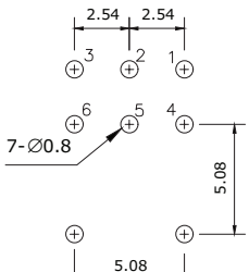
Recommended PCB Layout Top View
