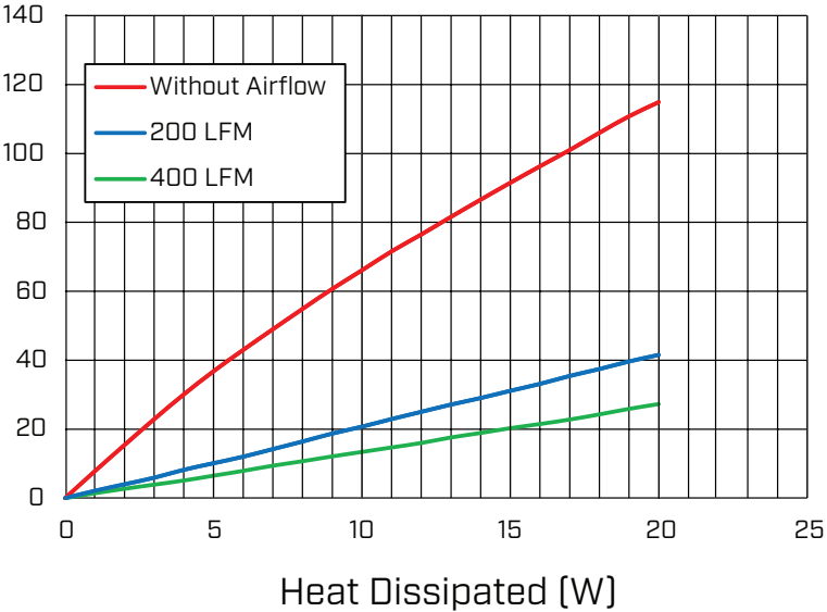
Mounting Surface Temperature Rise Above Ambient [°C]
