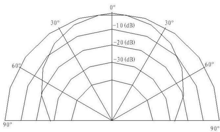
Directivity
