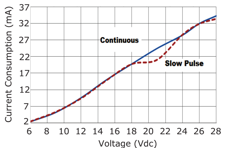
Voltage vs. Current Consumption
