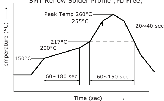
SMT Reflow Solder Profile (Pb Free)
