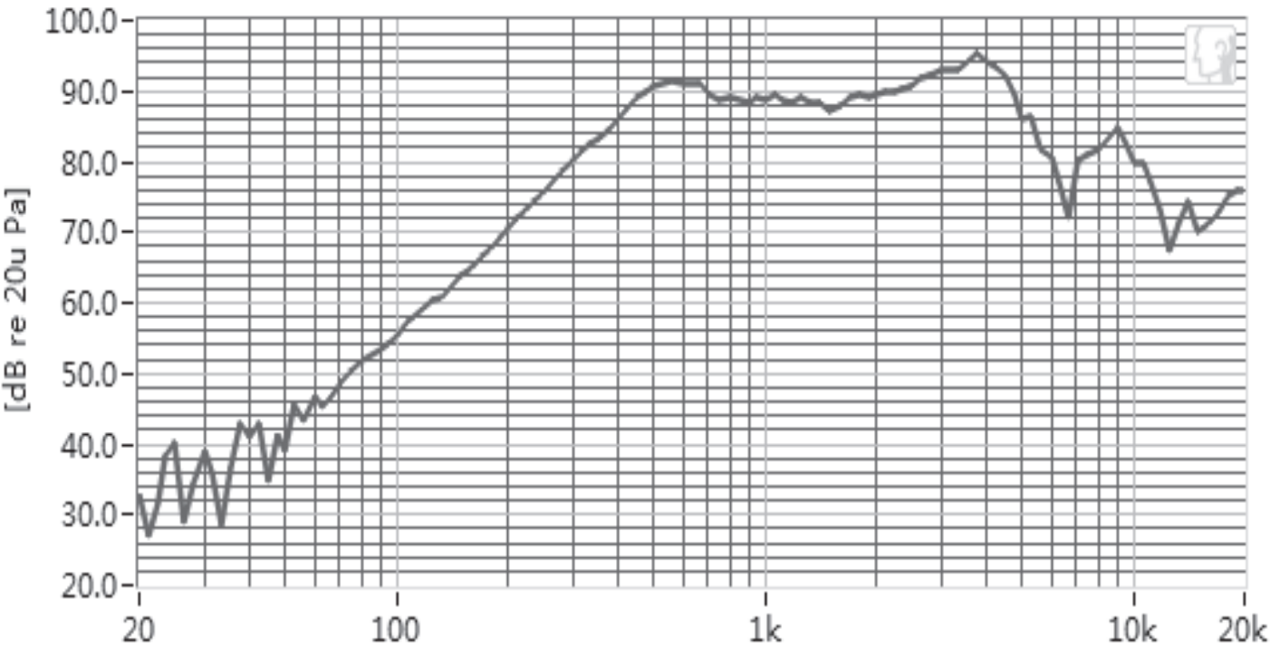
Frequency Response.Magn dB re 20.00μ PA (at 0.1 W / 0.1m)
