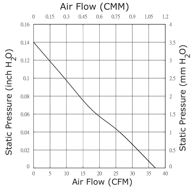
CFM-8015V-230-347
