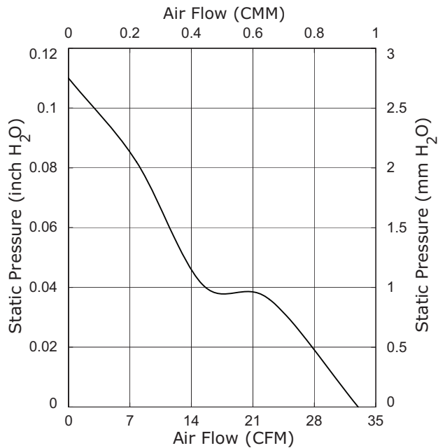
CFM-8025V-226-280
