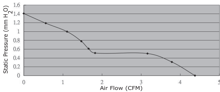
CFM-4020CF-235-114
