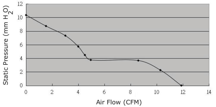
CFM-4020CF-195-342
