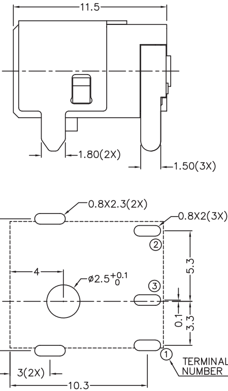
Recommended PCB Layout Top View
