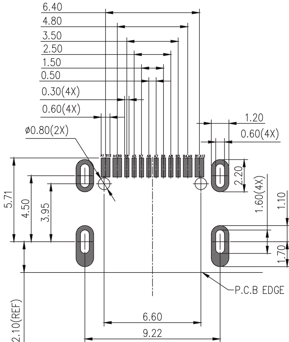
Recommended PCB Layout Top View
