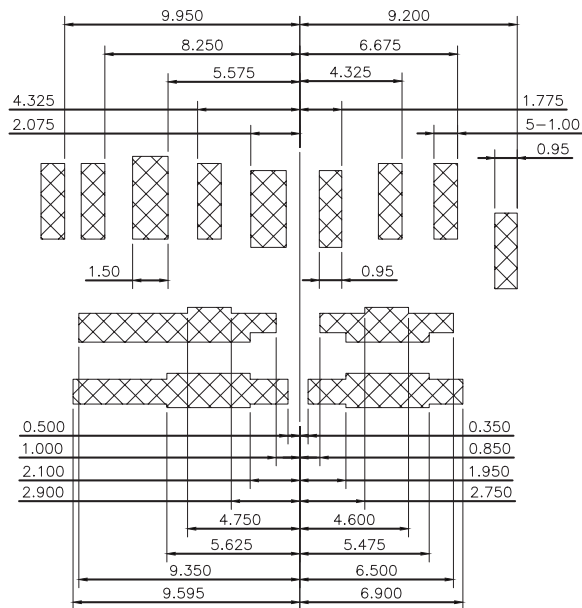
DETAIL J SCALE 2:1
