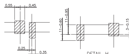
DETAIL G SCALE 4:1
