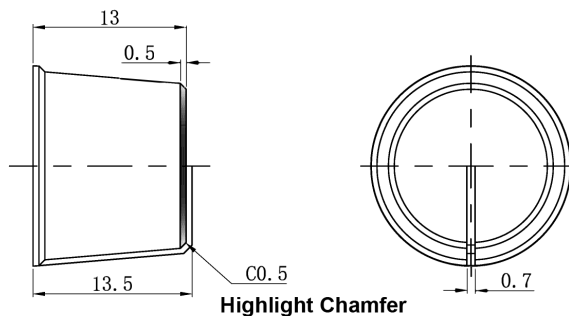
Highlight Chamfer
