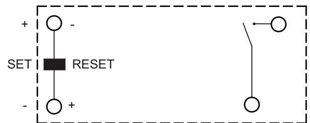
Wiring Diagram Bottom View
