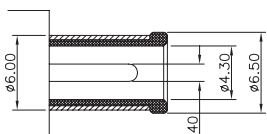
MATING PLUG Jack Insertion Depth: 9.1 mm
