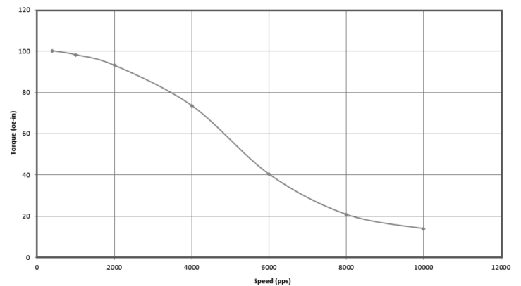
Same Sky P/N NEMA23-17-01PD-AMT112S Lin Engineering P/N WD-5718X-01P (1.8 Step Motor) 24 Vdc, 2.8 Amp/Phase, IB463, 1/2 Stepping
