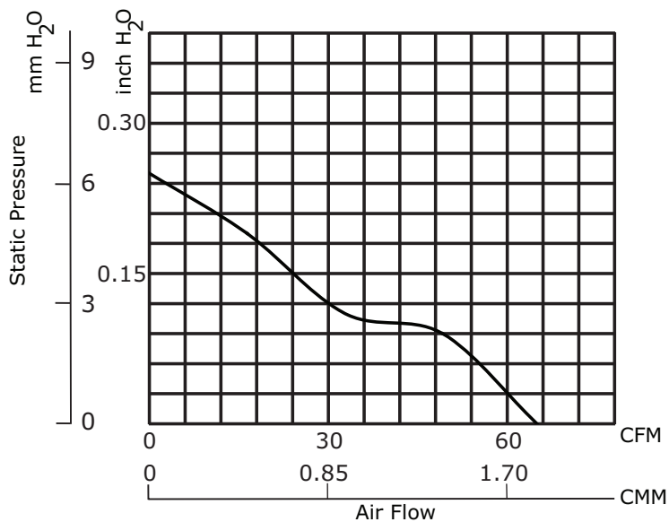
CFM-9225V-339-420
