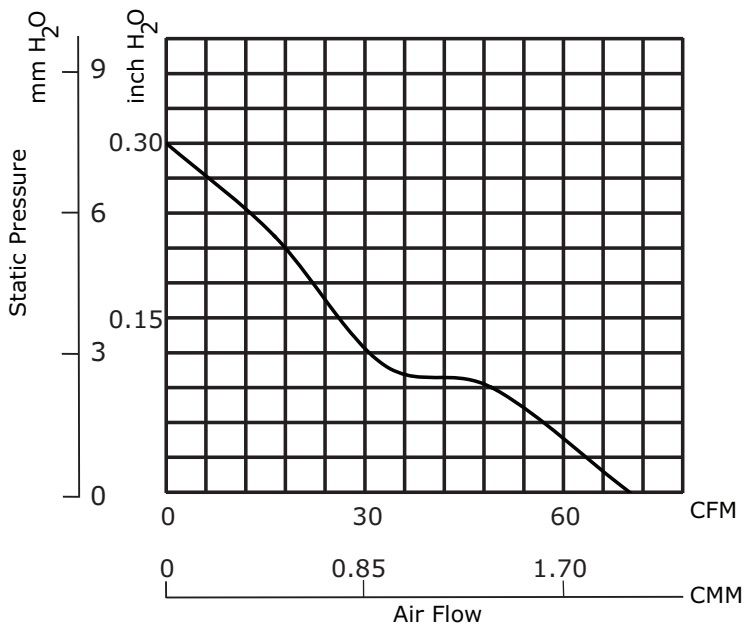
CFM-9225V-242-440
