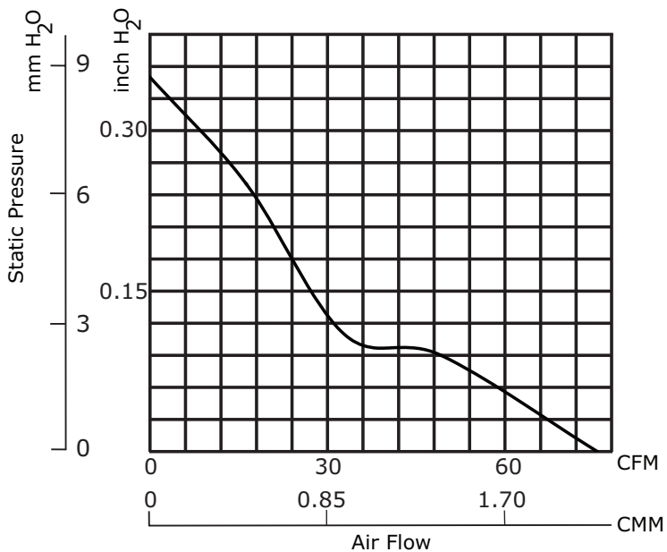
CFM-9225V-345-460
