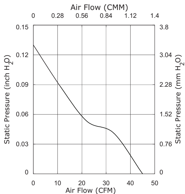
CFM-9225V-227-320
