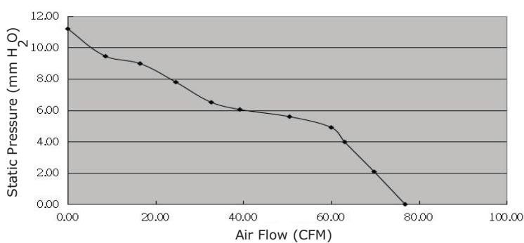
CFM-9238S-140-473
