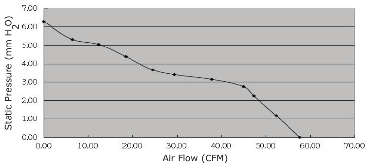
CFM-9238S-130-410
