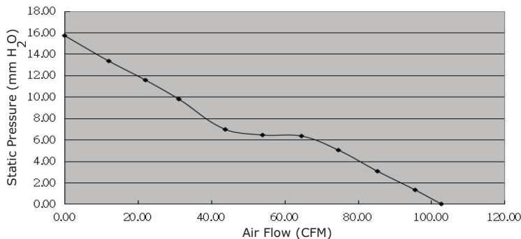
CFM-9232S-150-509
