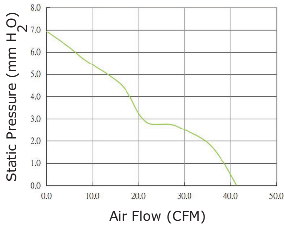
CFM-8025BG-160-484
