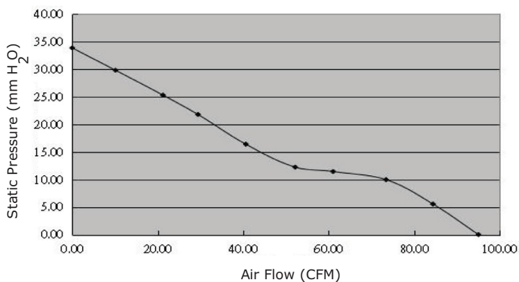
CFM-8025BG-490-592
