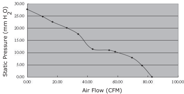
CFM-8025BG-180-546
