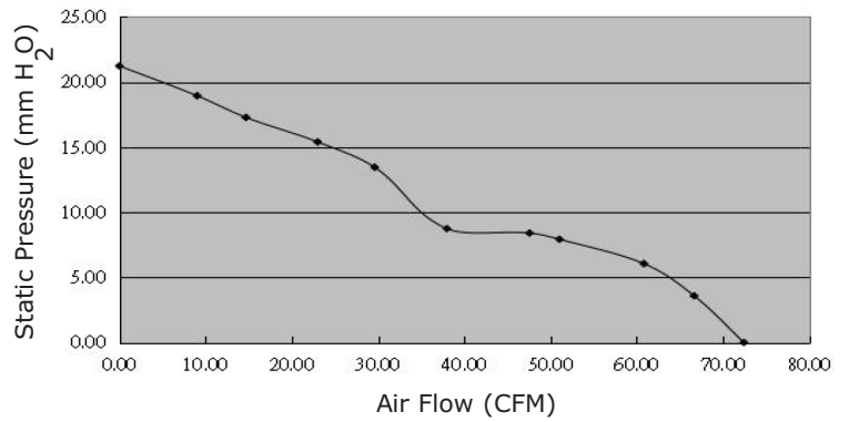
CFM-8025BG-190-572
