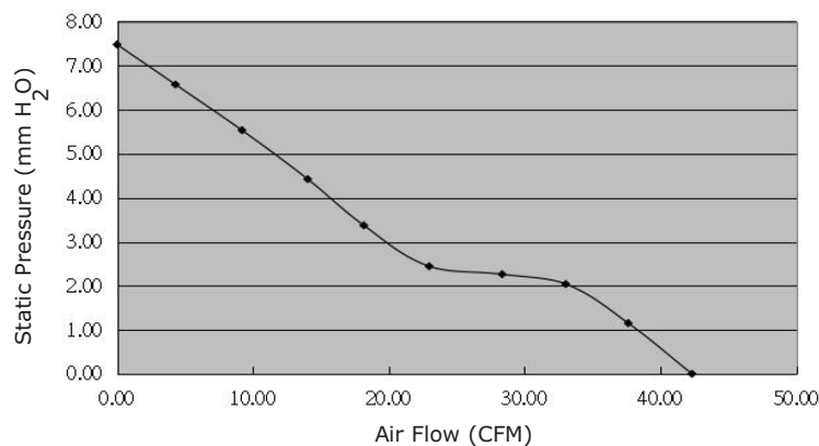
CFM-8025BG-440-383
