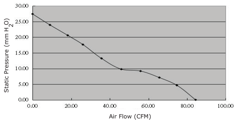
CFM-8025BG-480-561
