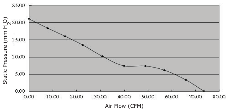
CFM-8025BG-490-592
