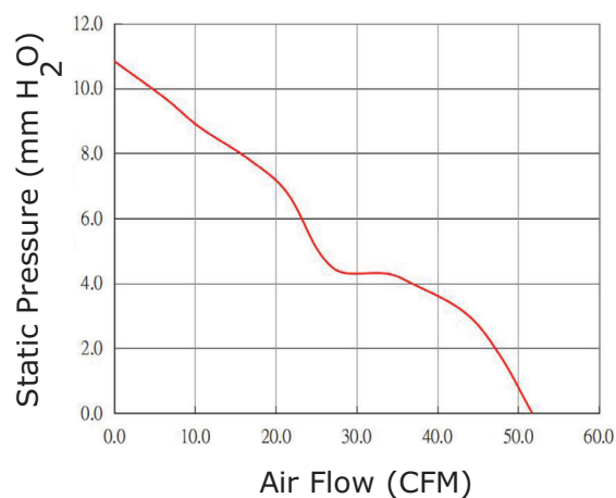
CFM-8025BG-270-517
