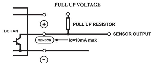
Figure 3 FG Signal Output Circuit: Open Collector
