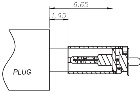
AFTER MATING
