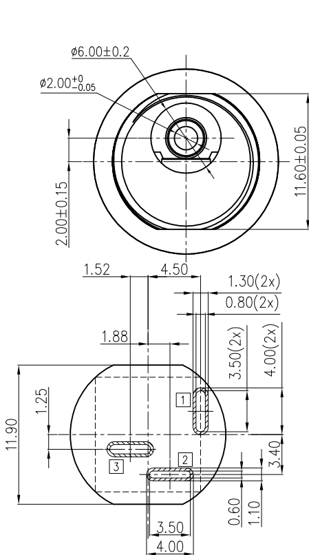
Recommended PCB Layout Bottom View
