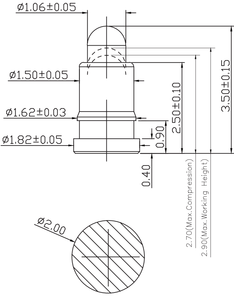
Recommended PCB Layout Top View
