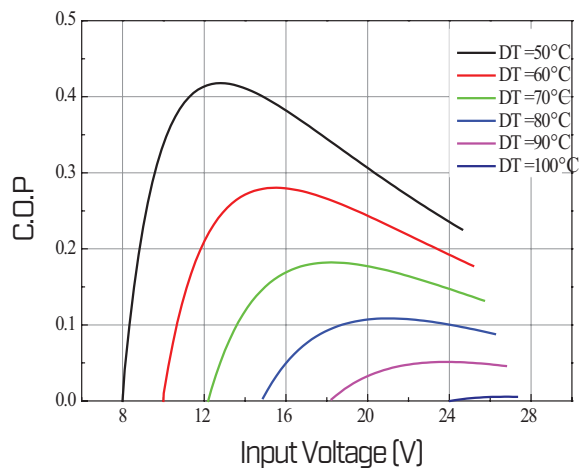
COP Vs. Input Voltage, V ( \Delta T=50\sim 100^\circ\text{C} )
