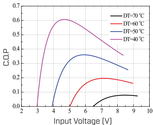
COP Vs. Input Voltage, V ( \Delta T = 40 \sim 70 °C)
