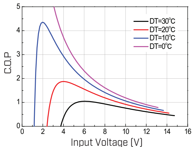
COP Vs. Input Voltage, V ( \Delta T=0\sim30^\circ\text{C} )
