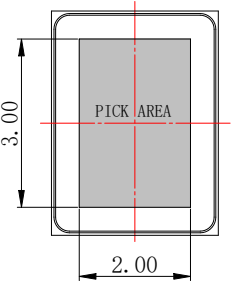
Recommended Vacuum Nozzle Pickup Top View
