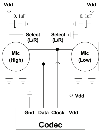
Dual Microphone
