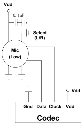
Single Microphone
