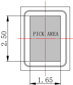
Recommended Vacuum Nozzle Pickup Top View
