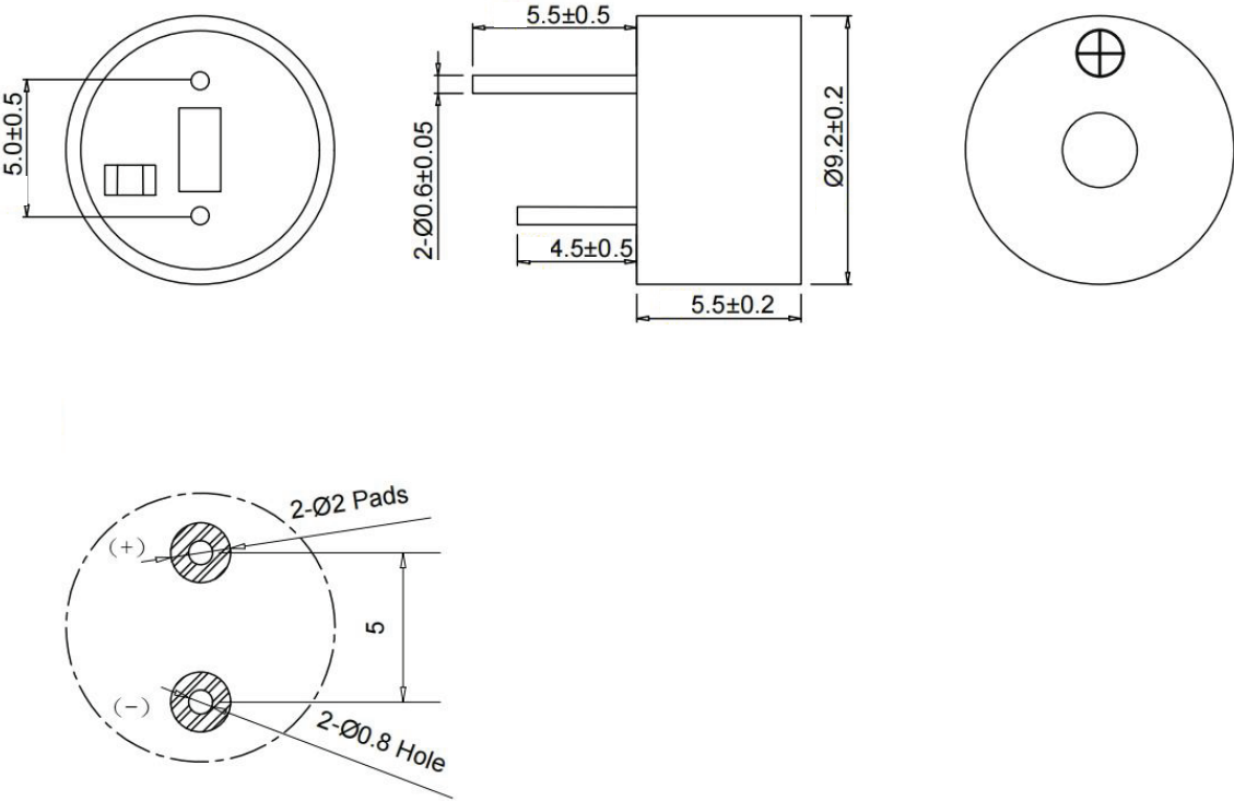
Recommended PCB Layout Top View
