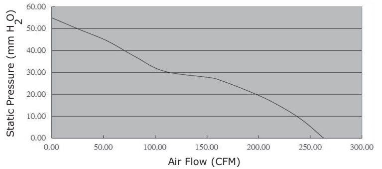
CFM-A238BF-280-680
