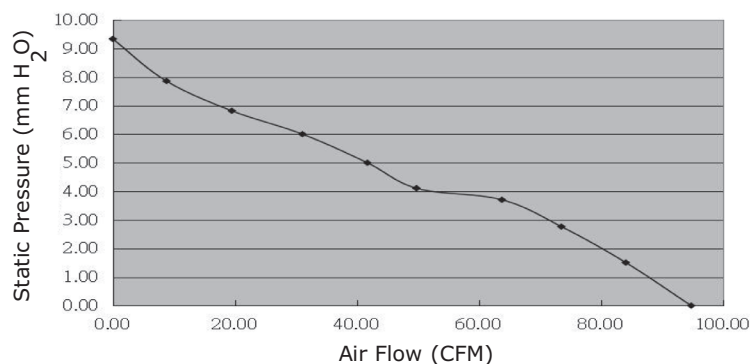
CFM-A225BF-453-604
