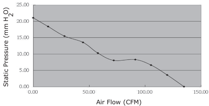
CFM-A238BF-440-524
