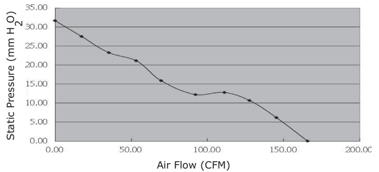
CFM-A238BF-450-573
