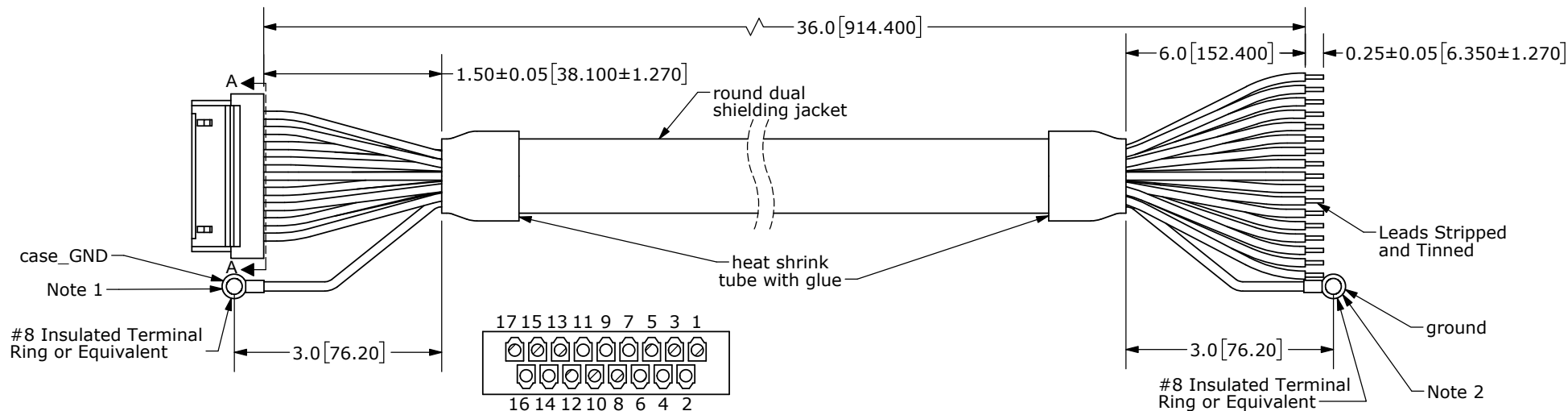
Connector Pinout
